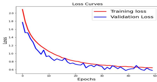
Figure 9: Loss Curves
