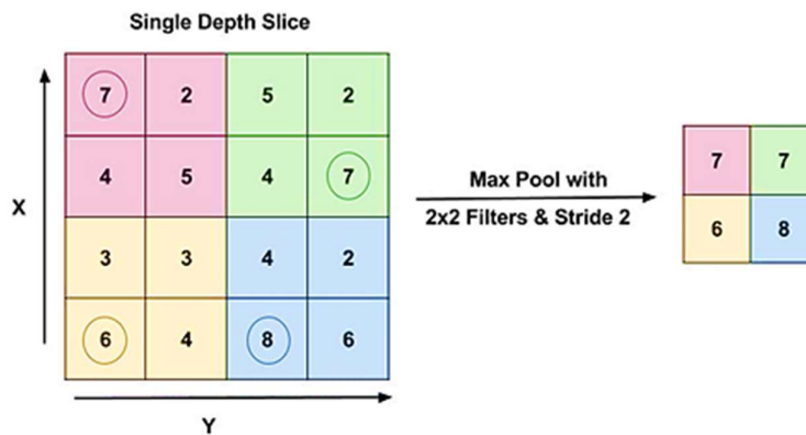
Figure 7: Be a very successful swimming pool layer with filter the max free in the 2 \times 2 place digits
