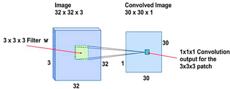
Figure 5: Convolution Operation by Sliding
