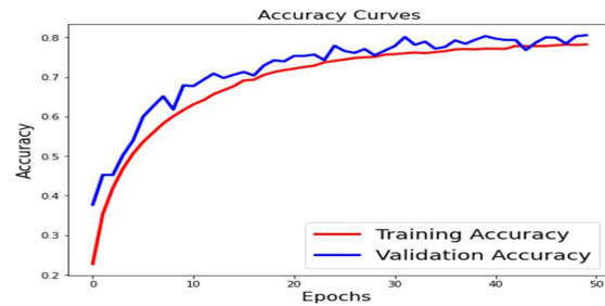
Figure 10: Accuracy Curves
