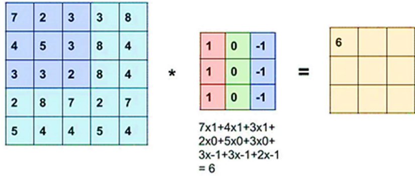
Figure 4: Convolutional Layer Neurons of CNN
