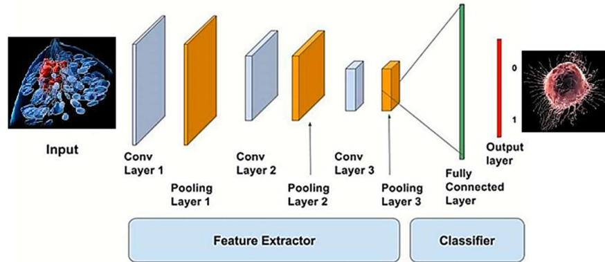
Figure 3: Convolutional Neural Network Image Detection Model
